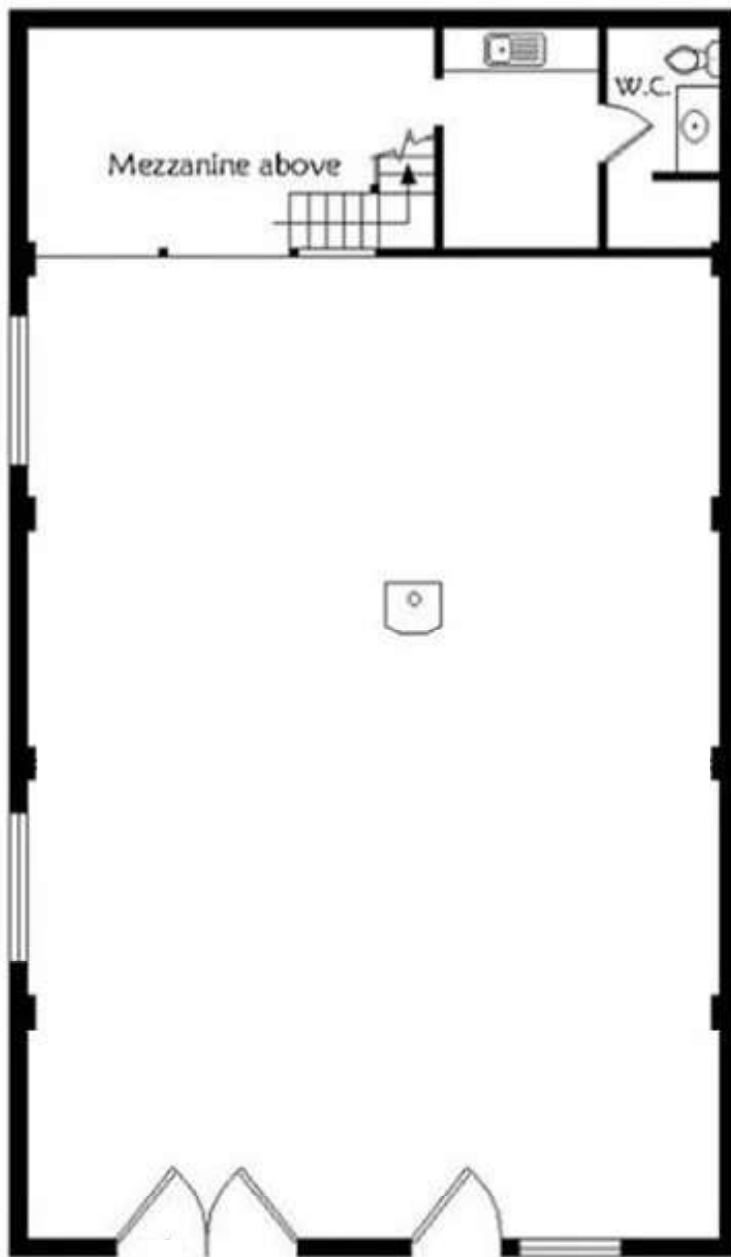
EXISTING GROUND FLOOR PLAN 91 Patrick St. West Hobart
