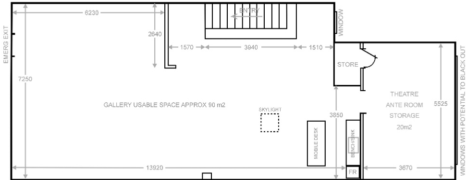
GALES GALLERY/PERFORMANCE/CLASS SPACE PLAN
